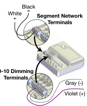
0-10V Dimming control wires (available for each load)
