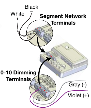
0-10V Dimming control wires (available for each load)
